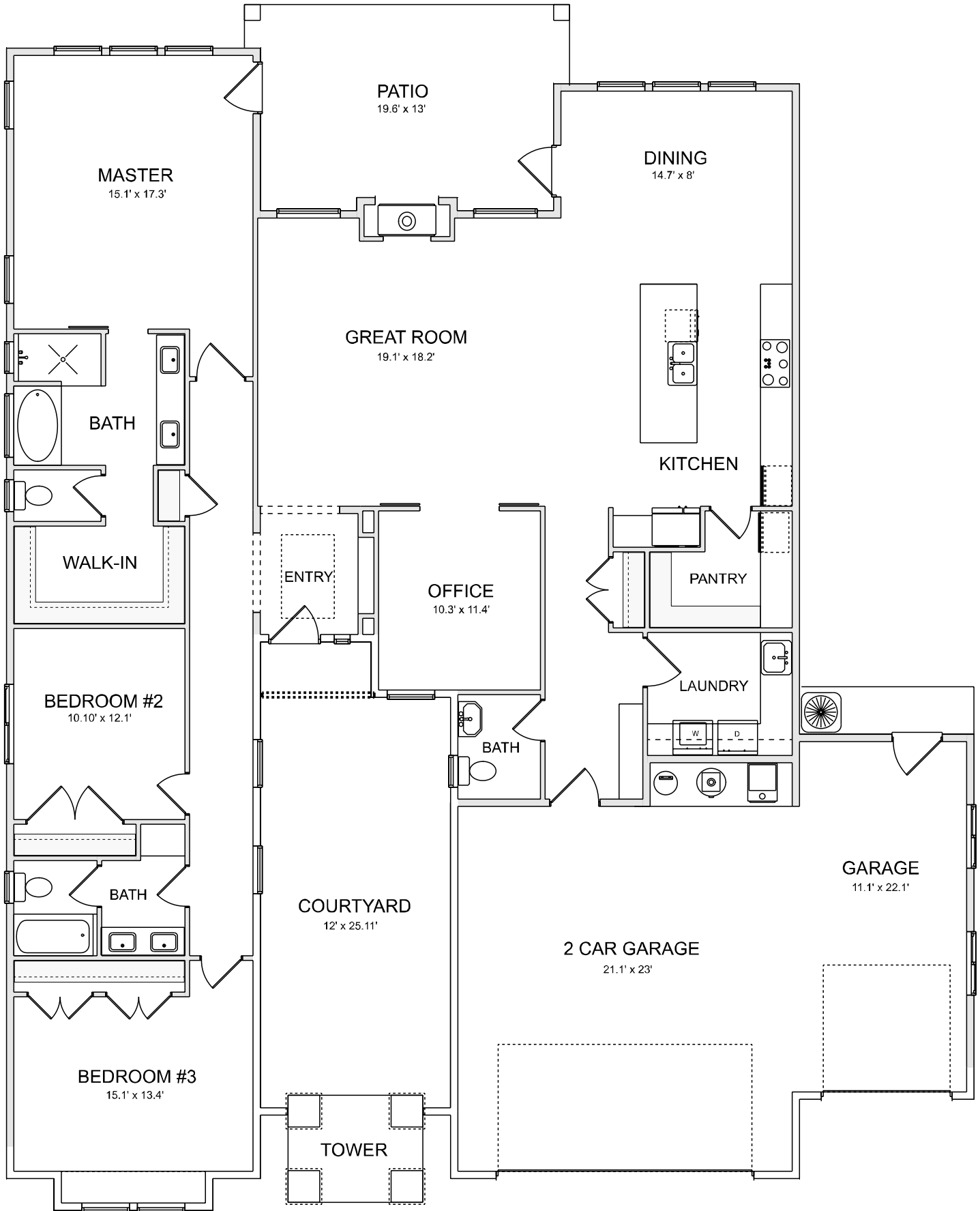
MAIN LEVEL FLOOR PLAN
